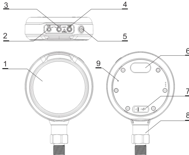
Figure 1 Basic Structure
