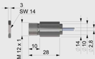
Sensing head
