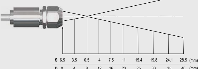
25:1 optics with CF-lens
