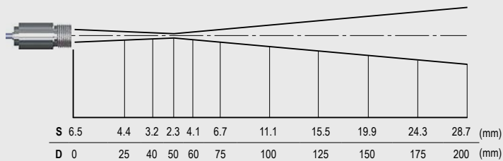
Optics CTi LT CF, D:S = 22:1 (far field = 6:1)
