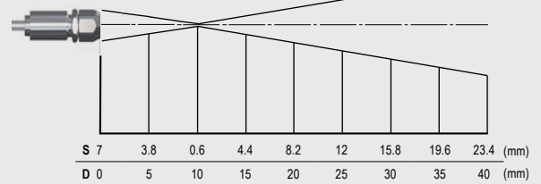
Optics CTi LT SF, D:S = 22:1, with additional CF lens (ACCTCF)/ far field = 1.5:1
